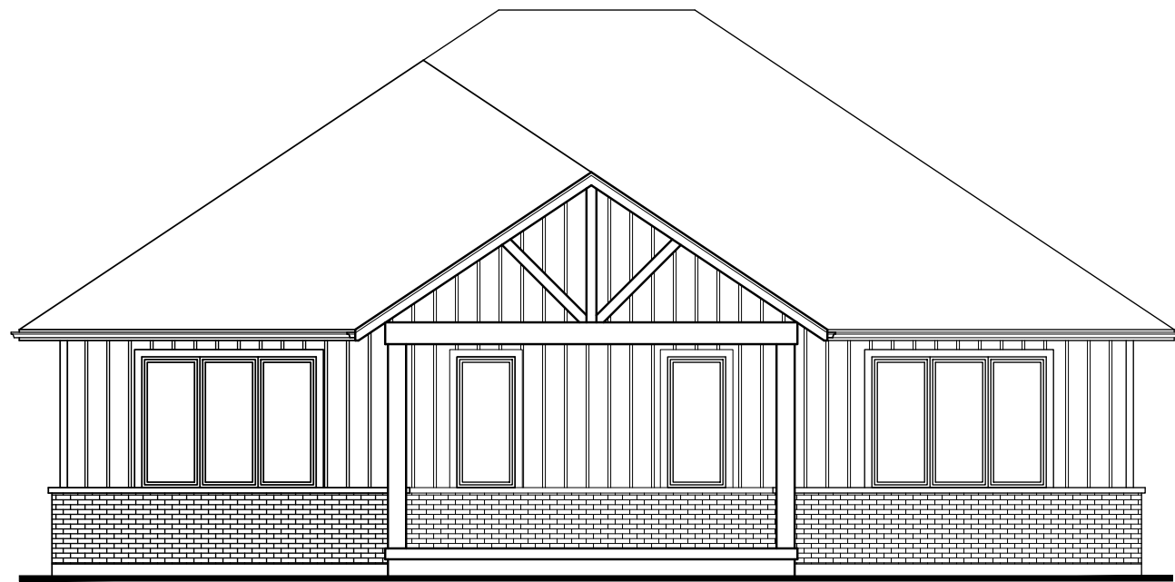
Rear Elevation
