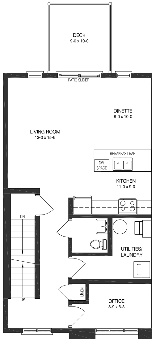
SECOND LEVEL PLAN
