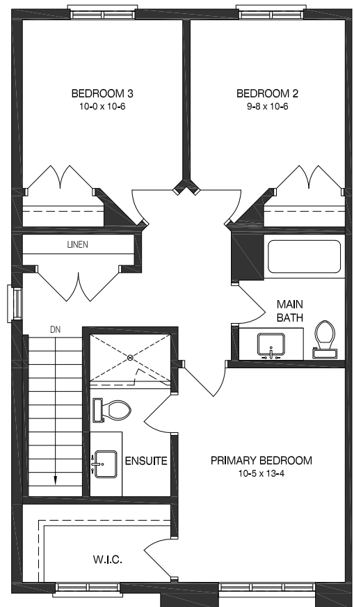
THIRD LEVEL PLAN
