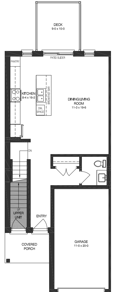
FIRST LEVEL PLAN
