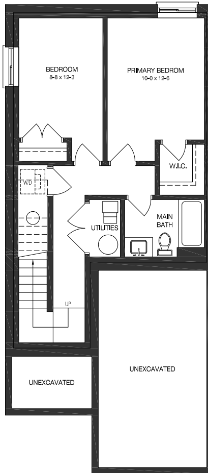
OPT. GROUND LEVEL PLAN
