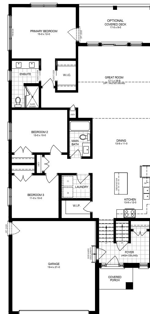
MAIN FLOOR
